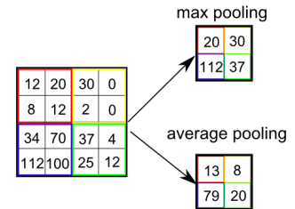
Figure 2.5: Mean and max pooling.
